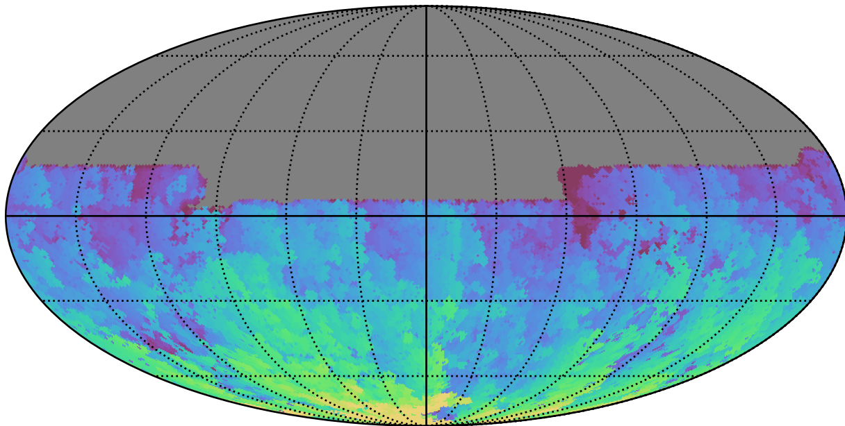
ddf_acor_sf15_lsf20_lsr50_v3.4_10yrs All sky u band: Max HA
