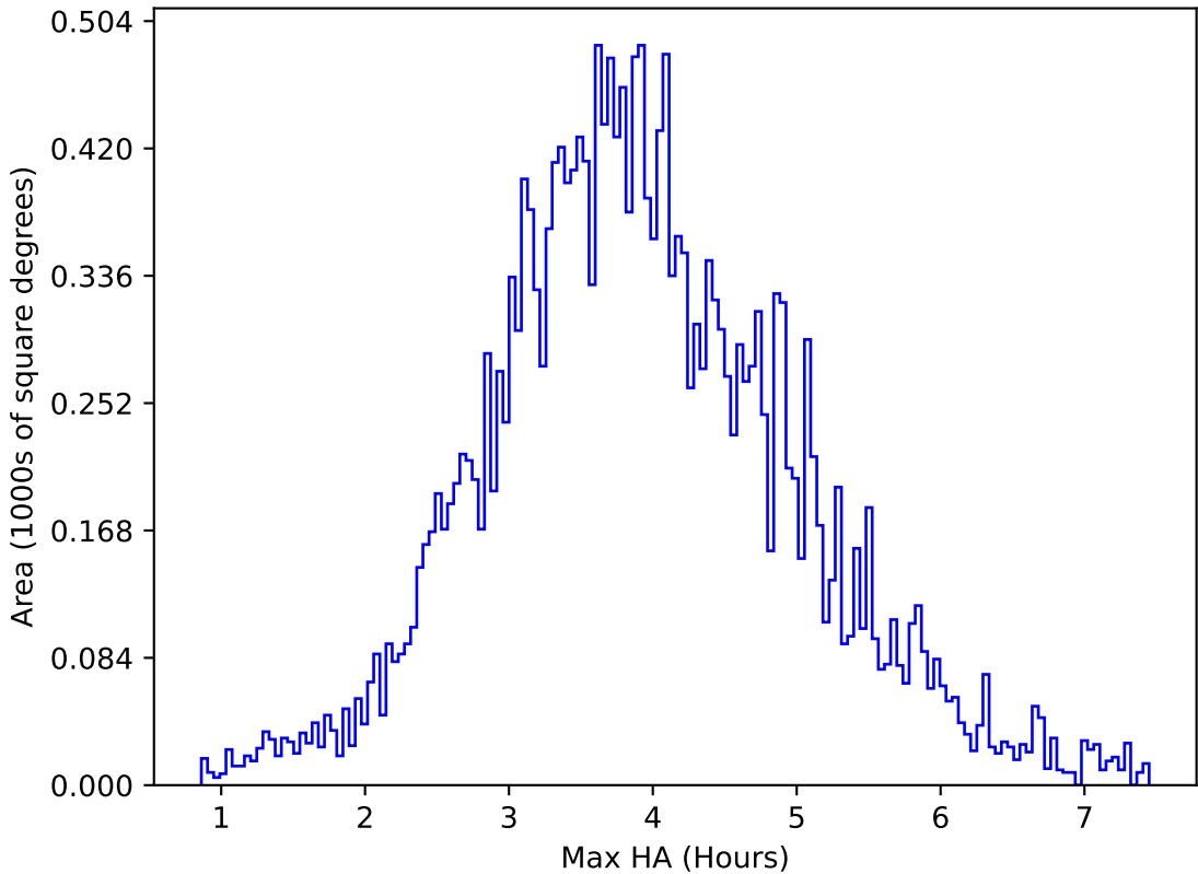
ddf_acor_sf15_lsf20_lsr50_v3.4_10yrs All sky u band: Max HA
