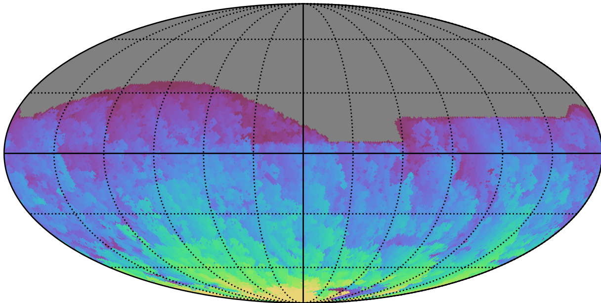
ddf_acor_sf15_lsf20_lsr50_v3.4_10yrs All sky r band: Max HA
