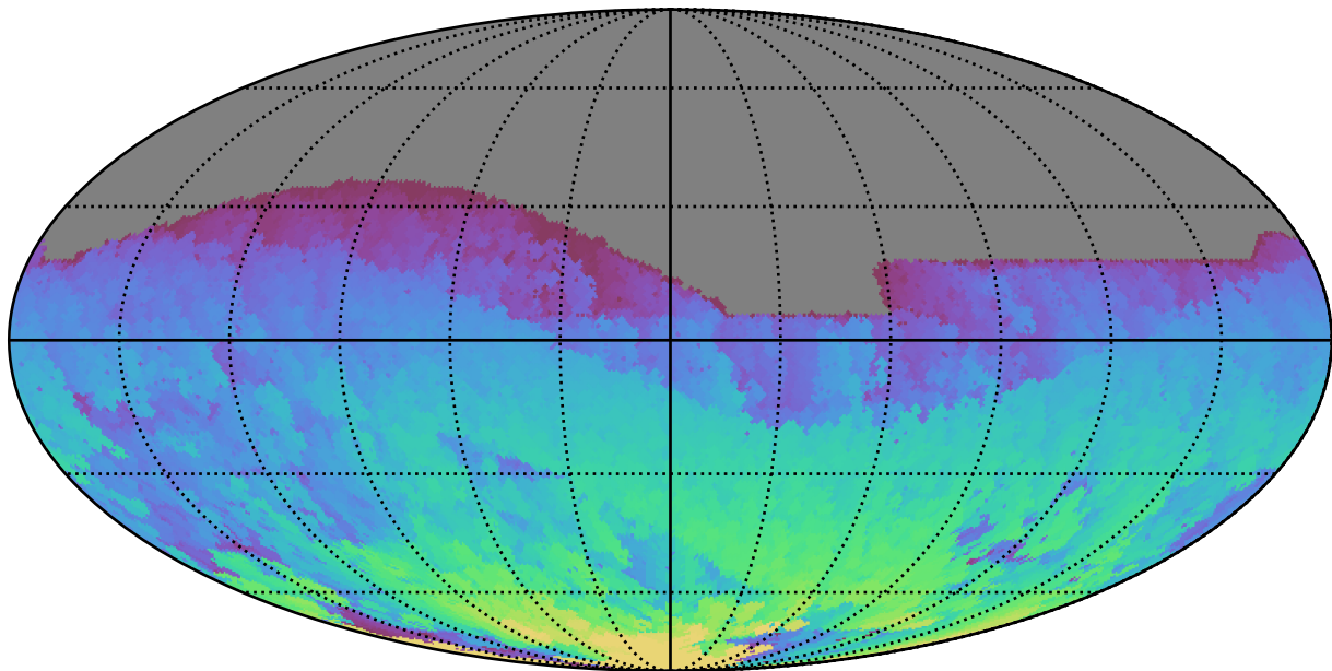
ddf_acor_sf15_lsf20_lsr50_v3.4_10yrs All sky i band: Max HA
