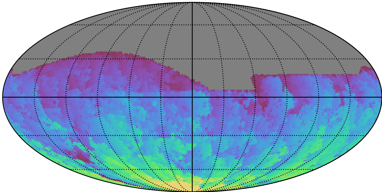
ddf_acor_sf15_lsf20_lsr50_v3.4_10yrs All sky g band: Max HA
