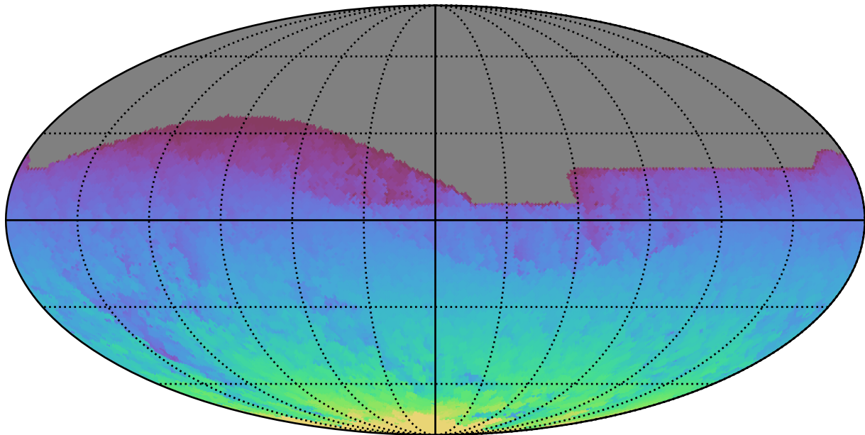
ddf_acor_sf15_lsf20_lsr50_v3.4_10yrs All sky all bands: Max HA
