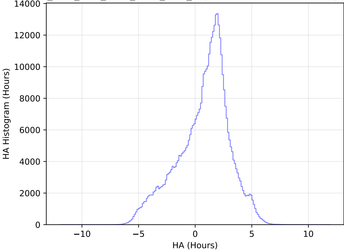
ddf_acor_sf15_ls20_lsr50_v3.4_10yrs WFD z band: HA Histogram
