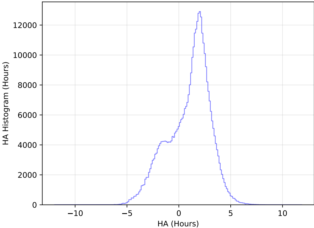
ddf_acor_sf15_lsf20_lsr50_v3.4_10yrs WFD y band: HA Histogram
