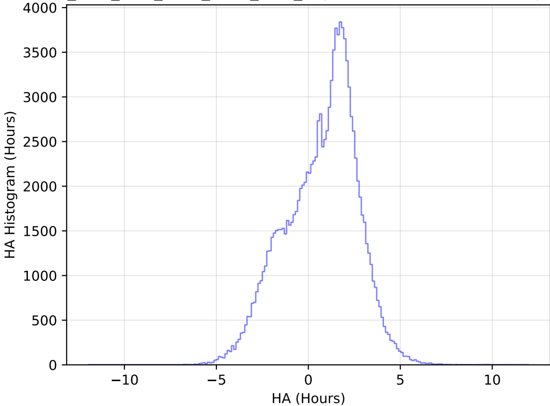
ddf_acor_sf15_lsf20_lsr50_v3.4_10yrs WFD u band: HA Histogram
