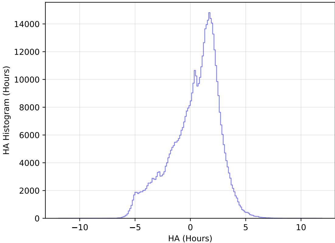
ddf_acor_sf15_lsf20_lsr50_v3.4_10yrs WFD r band: HA Histogram
