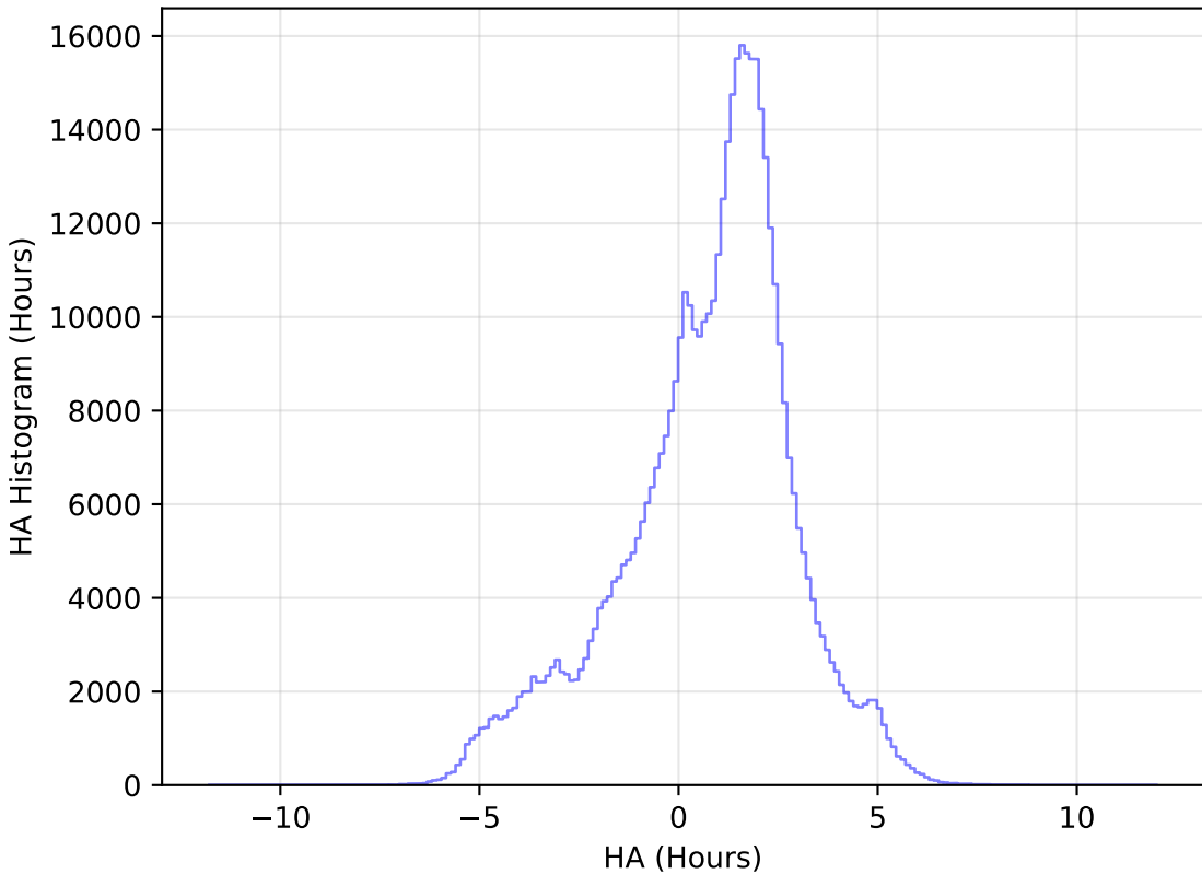
ddf_acor_sf15_lsf20_lsr50_v3.4_10yrs WFD i band: HA Histogram
