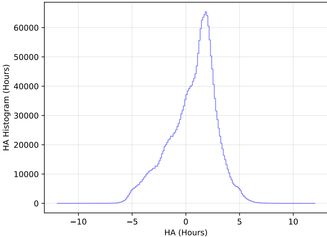
ddf_acor_sf15_lsf20_lsr50_v3.4_10yrs WFD all bands: HA Histogram
