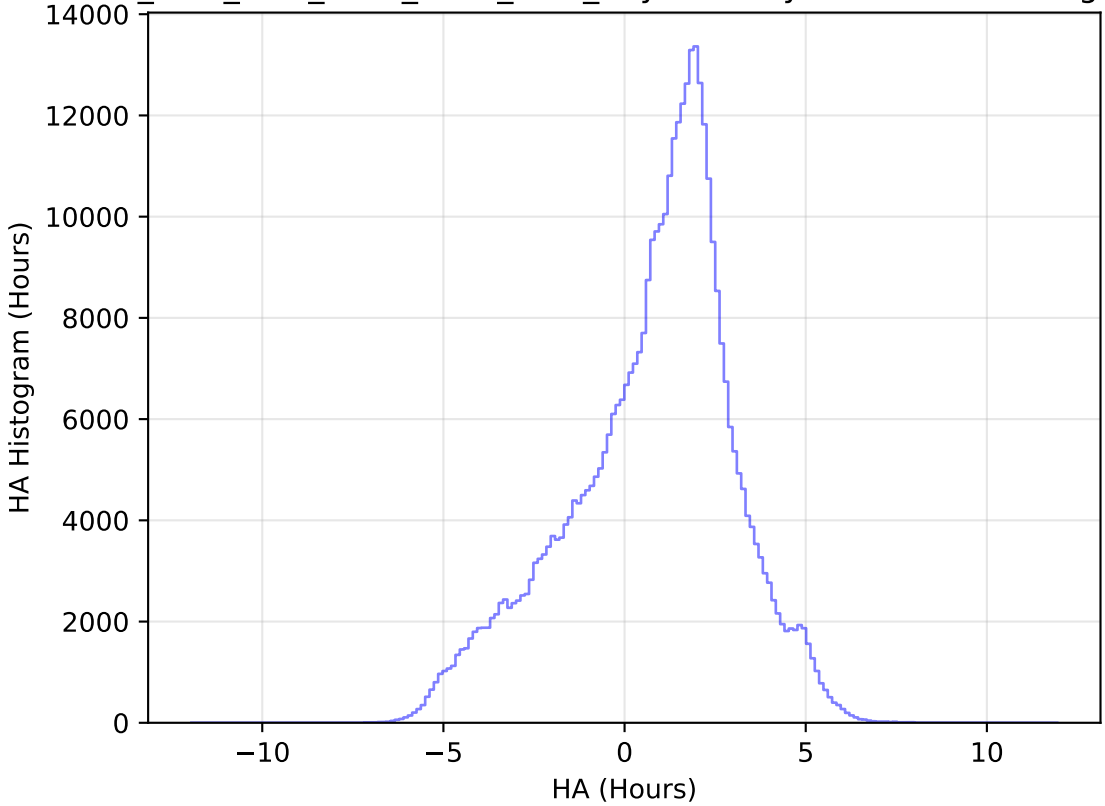
ddf_acor_sf15_lsf20_lsr50_v3.4_10yrs All sky z band: HA Histogram
