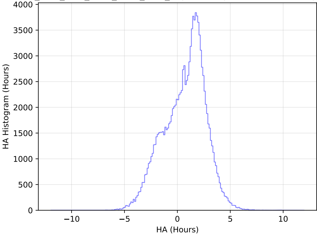
ddf_acor_sf15_lsf20_lsr50_v3.4_10yrs All sky u band: HA Histogram
