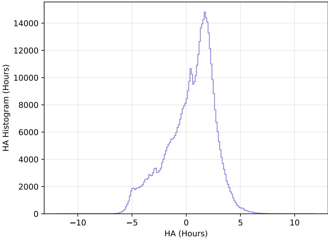
ddf_acor_sf15_lsf20_lsr50_v3.4_10yrs All sky r band: HA Histogram
