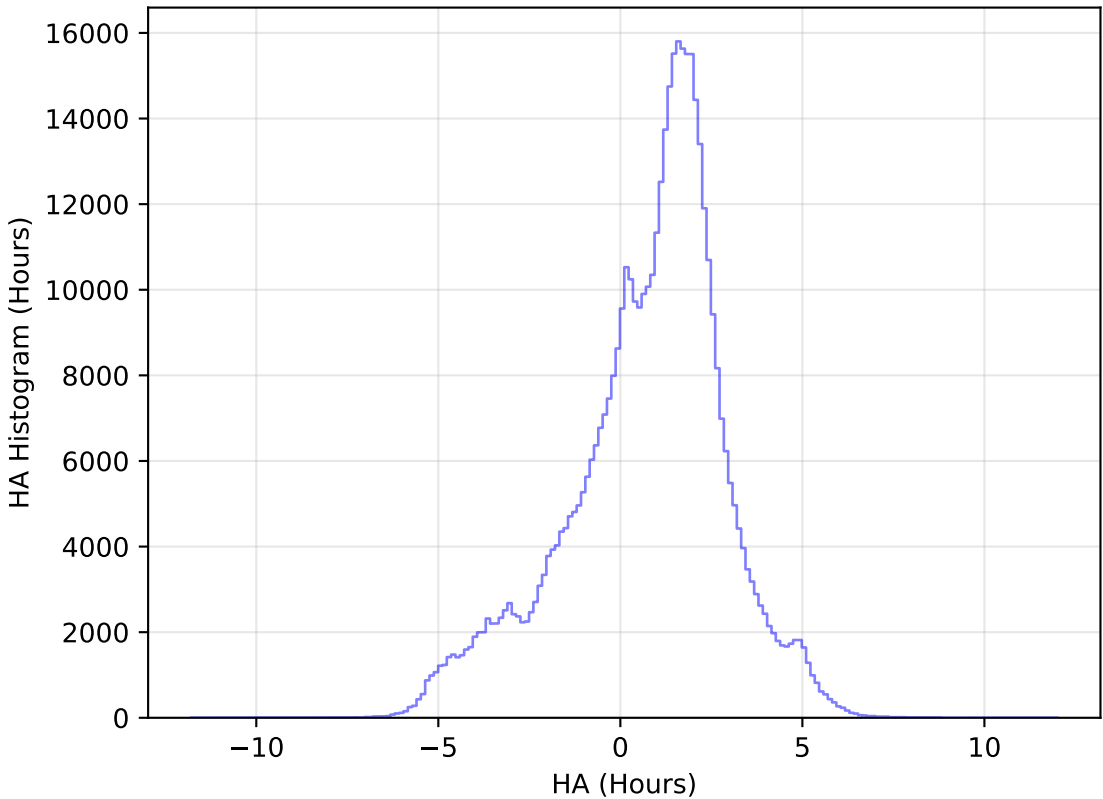
ddf_acor_sf15_lsf20_lsr50_v3.4_10yrs All sky i band: HA Histogram
