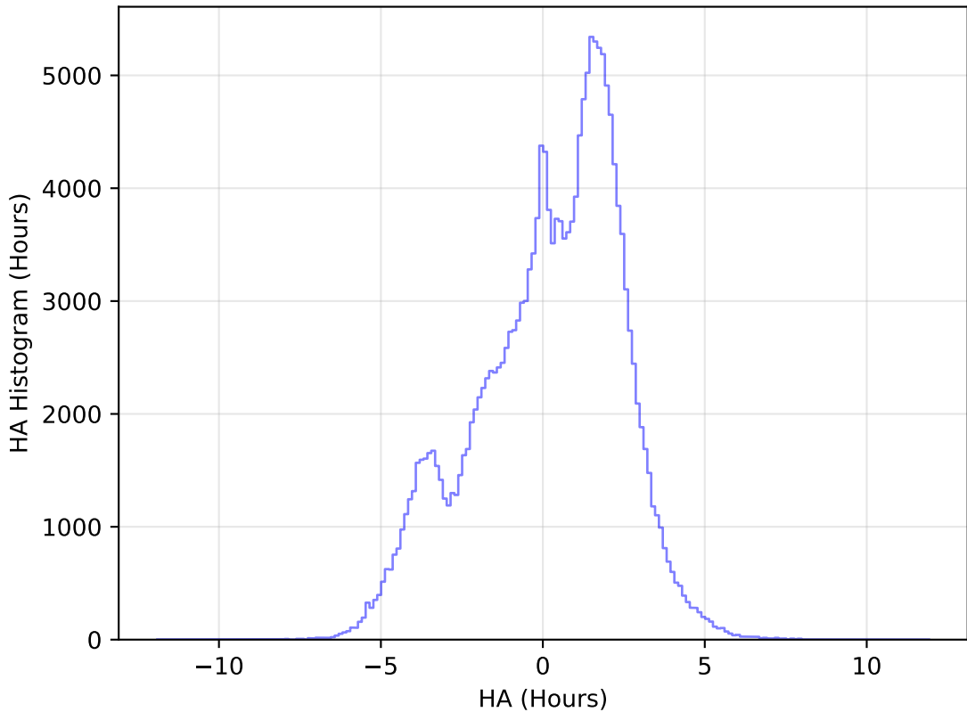
ddf_acor_sf15_lsf20_lsr50_v3.4_10yrs All sky g band: HA Histogram
