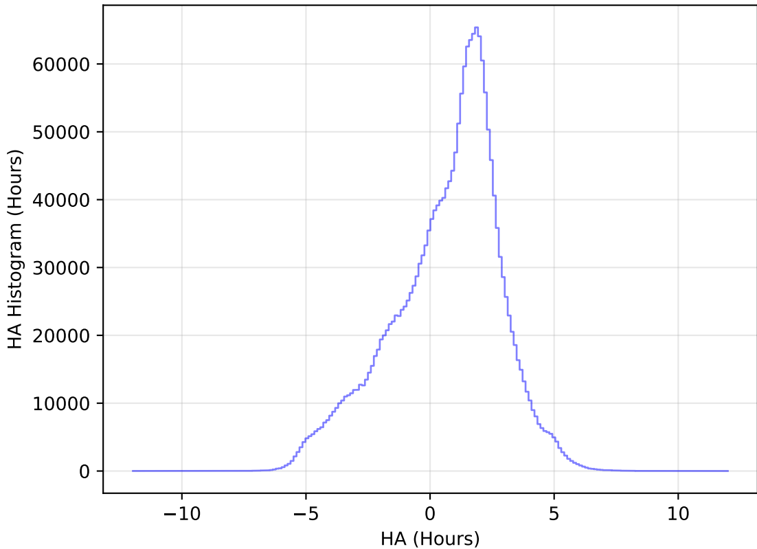
ddf_acor_sf15_lsf20_lsr50_v3.4_10yrs All sky all bands: HA Histogram
