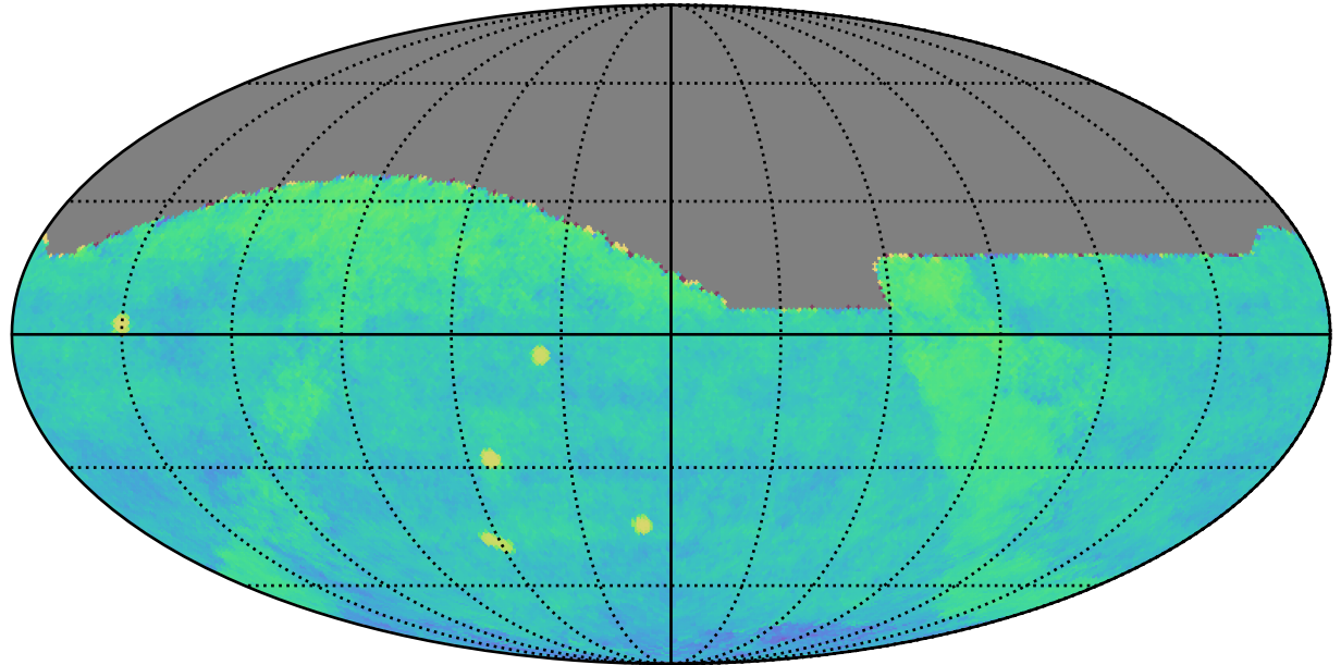
ddf_acor_sf15_lsf20_lsr50_v3.4_10yrs gri All sky: Fraction of visits in pairs (10-60 min)
