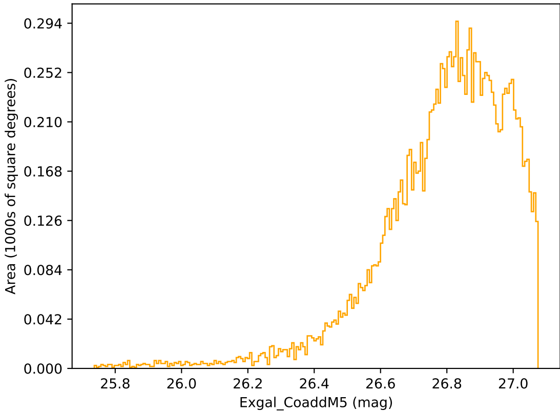
ddf_acor_sf15_lsf20_lsr50_v3.4_10yrs WFD r band: Exgal_CoaddM5
