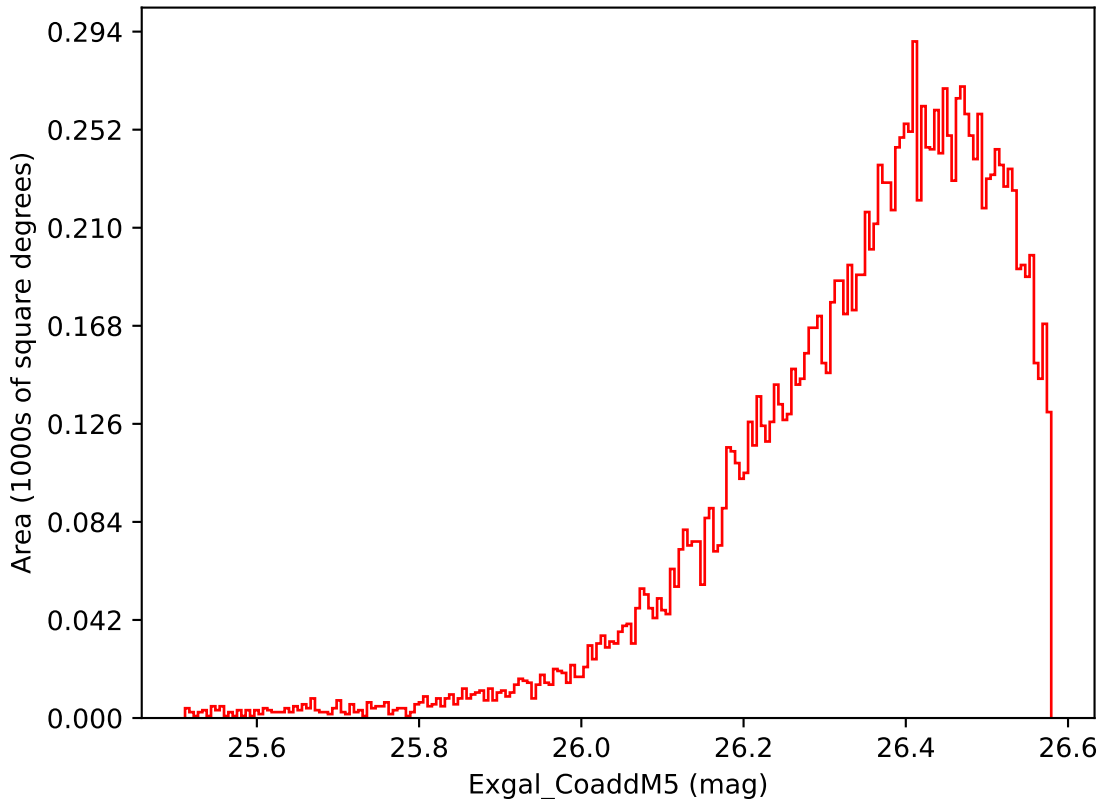
ddf_acor_sf15_lsf20_lsr50_v3.4_10yrs WFD i band: Exgal_CoaddM5
