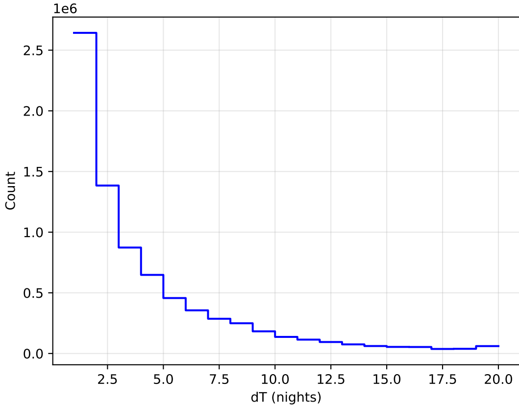
ddf_acor_sf15_lsf20_lsr50_v3.4_10yrs WFD all bands: DeltaNight Histogram
