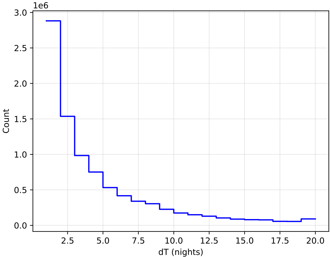
ddf_acor_sf15_lsf20_lsr50_v3.4_10yrs All sky all bands: DeltaNight Histogram
