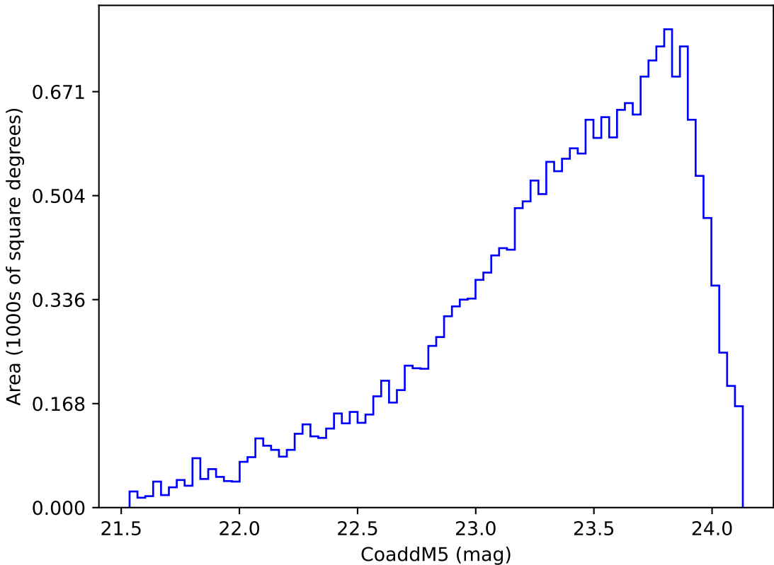
ddf_acor_sf15_lsf20_lsr50_v3.4_10yrs Yr 3-4 y band: CoaddM5
