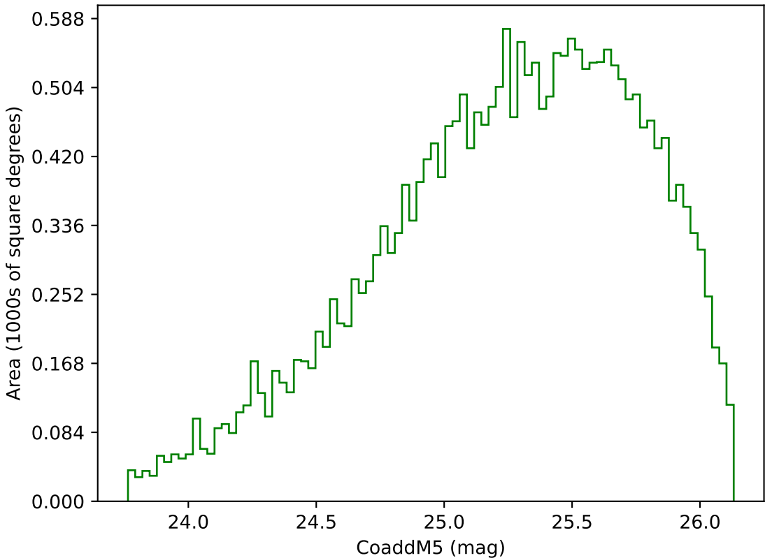
ddf_acor_sf15_lsf20_lsr50_v3.4_10yrs Yr 3-4 g band: CoaddM5
