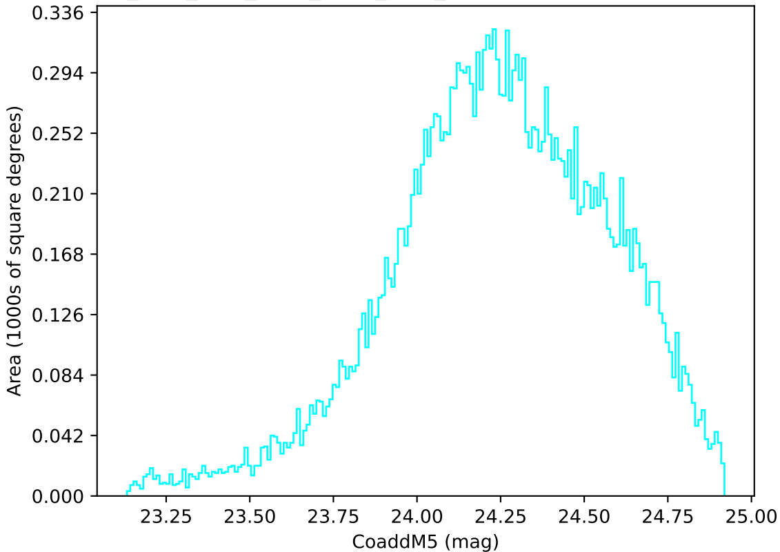
ddf_acor_sf15_lsf20_lsr50_v3.4_10yrs Yr 1 u band: CoaddM5
