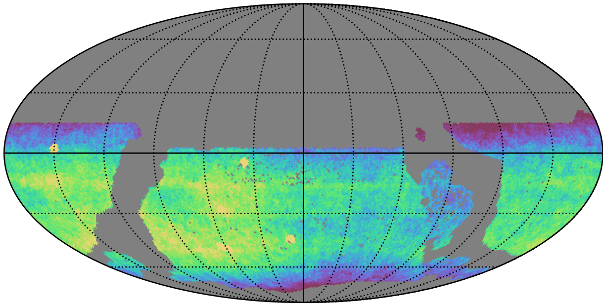
ddf_acor_sf15_lsf20_lsr50_v3.4_10yrs WFD z band: CoaddM5
