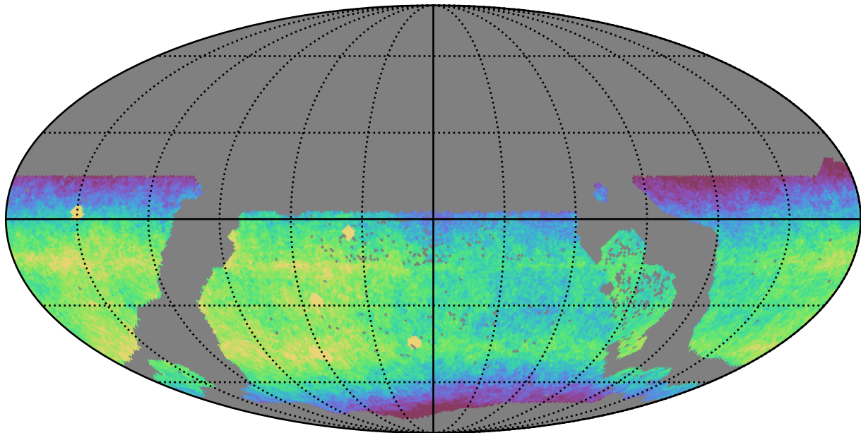
ddf_acor_sf15_lsf20_lsr50_v3.4_10yrs WFD i band: CoaddM5
