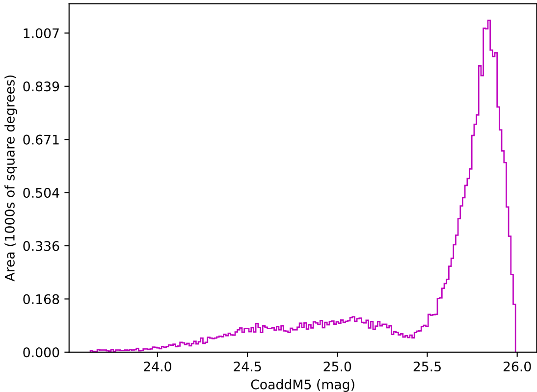
ddf_acor_sf15_lsf20_lsr50_v3.4_10yrs All sky z band: CoaddM5
