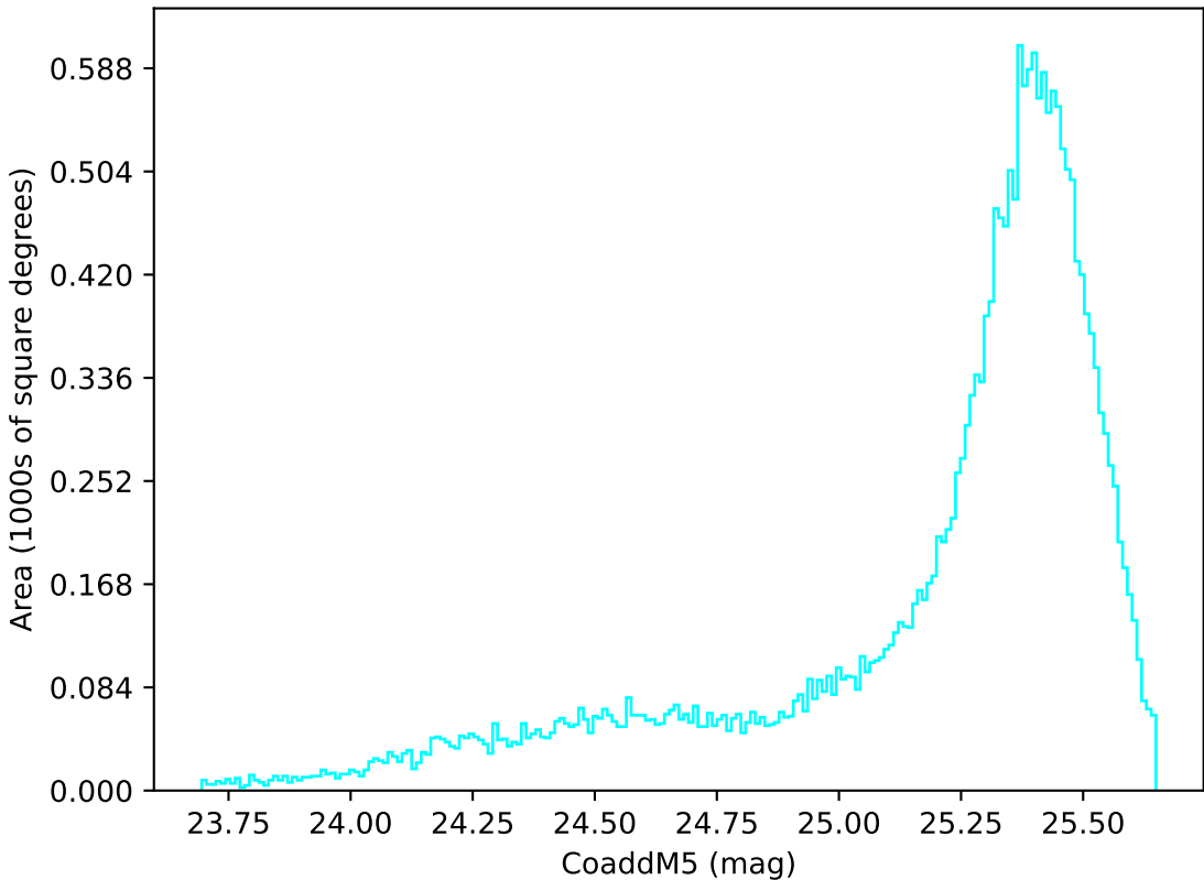
ddf_acor_sf15_lsf20_lsr50_v3.4_10yrs All sky u band: CoaddM5
