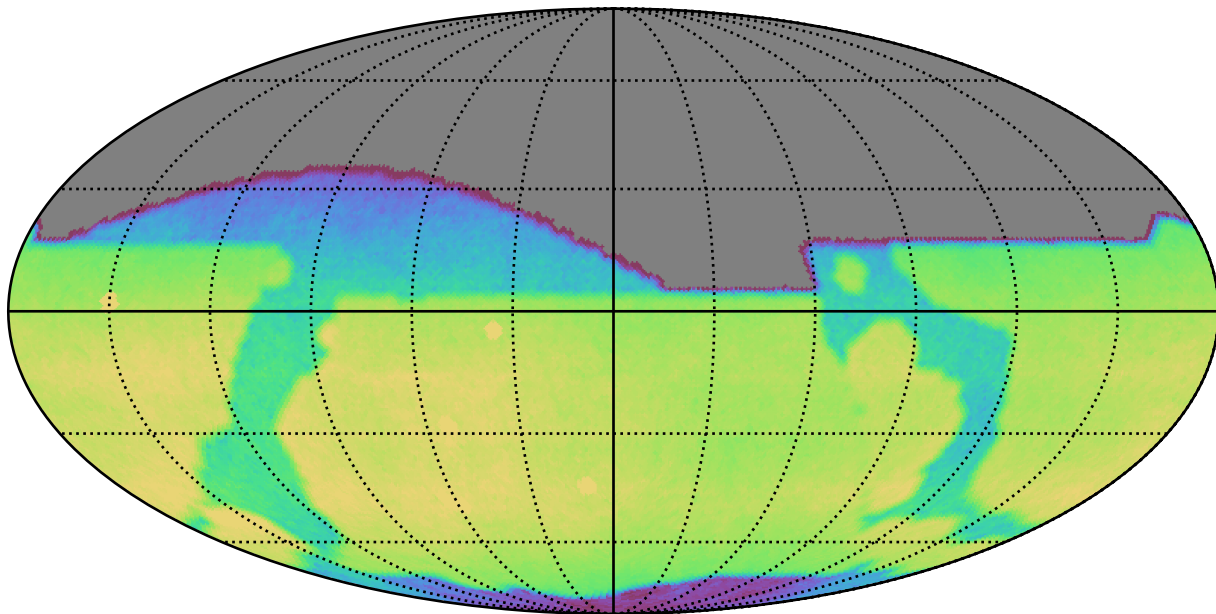
ddf_acor_sf15_lsf20_lsr50_v3.4_10yrs All sky r band: CoaddM5
