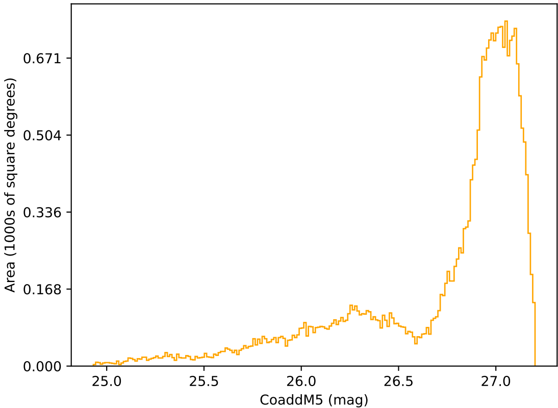
ddf_acor_sf15_lsf20_lsr50_v3.4_10yrs All sky r band: CoaddM5
