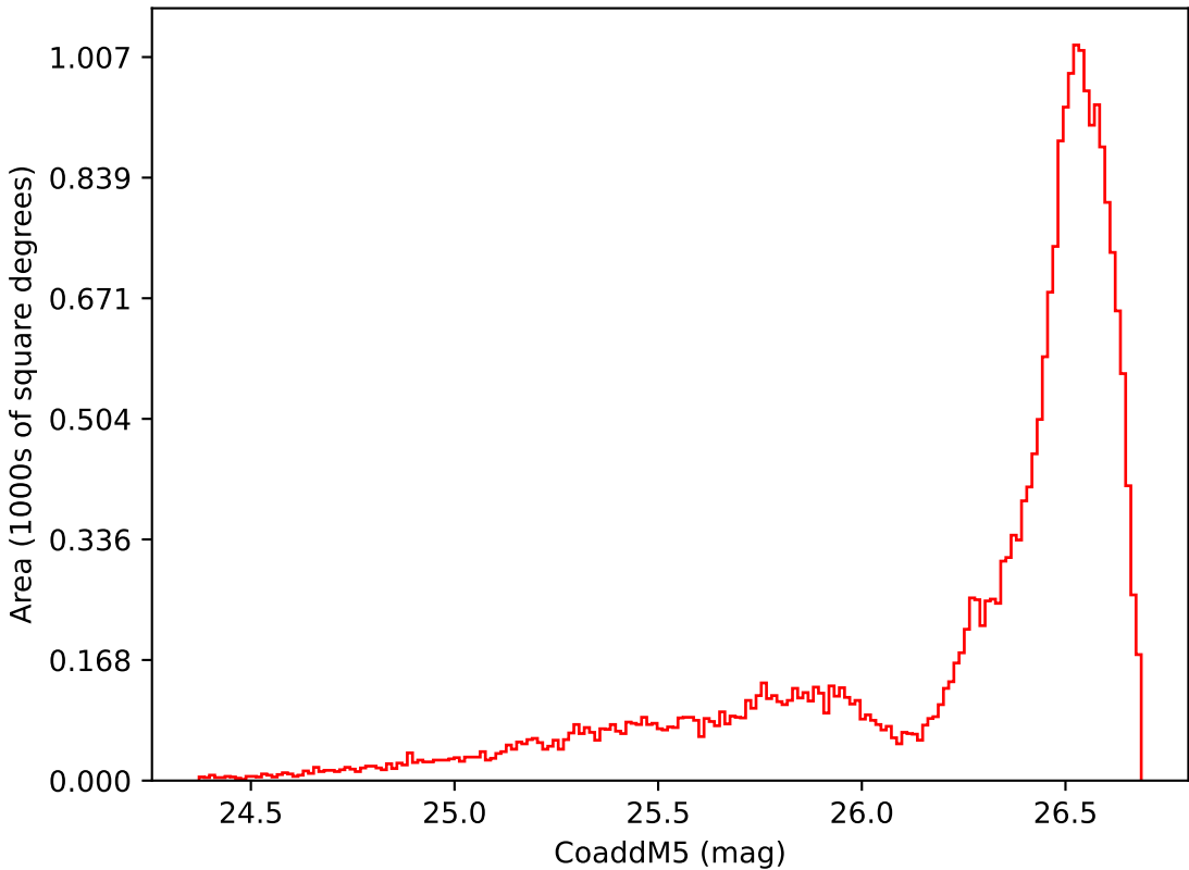
ddf_acor_sf15_lsf20_lsr50_v3.4_10yrs All sky i band: CoaddM5
