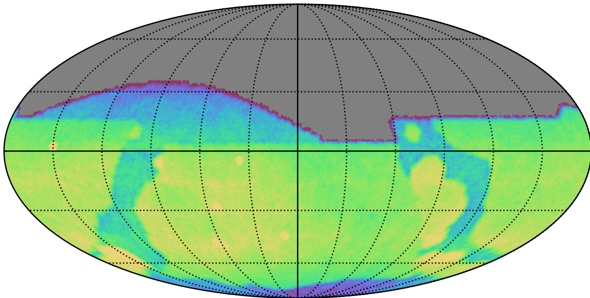
ddf_acor_sf15_lsf20_lsr50_v3.4_10yrs All sky g band: CoaddM5
