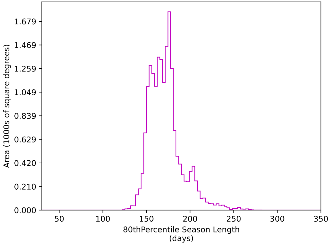
ddf_acor_sf15_lsf20_lsr50_v3.4_10yrs WFD z band: 80thPercentile Season Length
