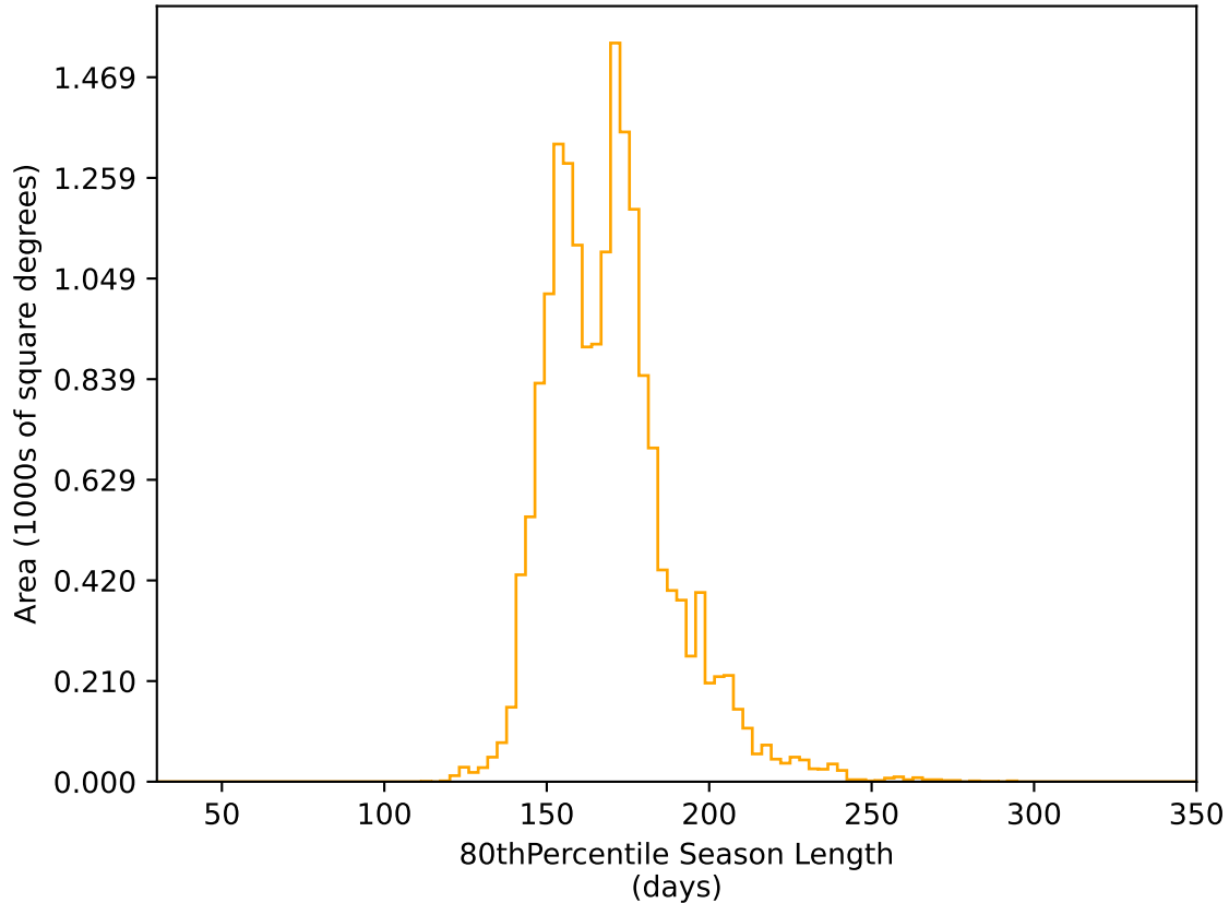
ddf_acor_sf15_lsf20_lsr50_v3.4_10yrs WFD r band: 80thPercentile Season Length
