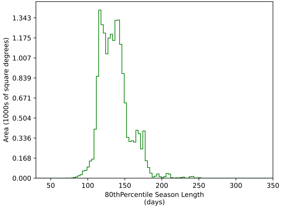
ddf_acor_sf15_lsf20_lsr50_v3.4_10yrs WFD g band: 80thPercentile Season Length
