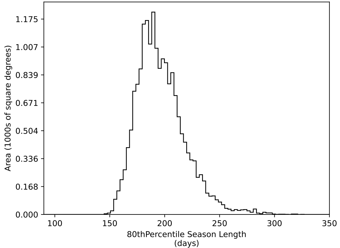
ddf_acor_sf15_lsf20_lsr50_v3.4_10yrs WFD all bands: 80thPercentile Season Length
