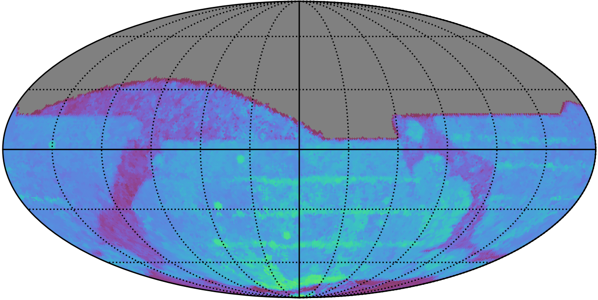
ddf_acor_sf15_lsf20_lsr50_v3.4_10yrs All sky z band: 80thPercentile Season Length
