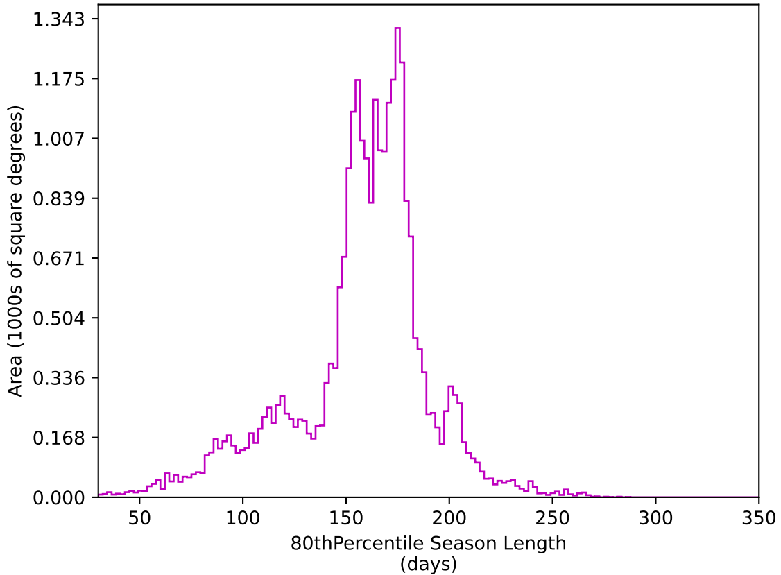
ddf_acor_sf15_lsf20_lsr50_v3.4_10yrs All sky z band: 80thPercentile Season Length
