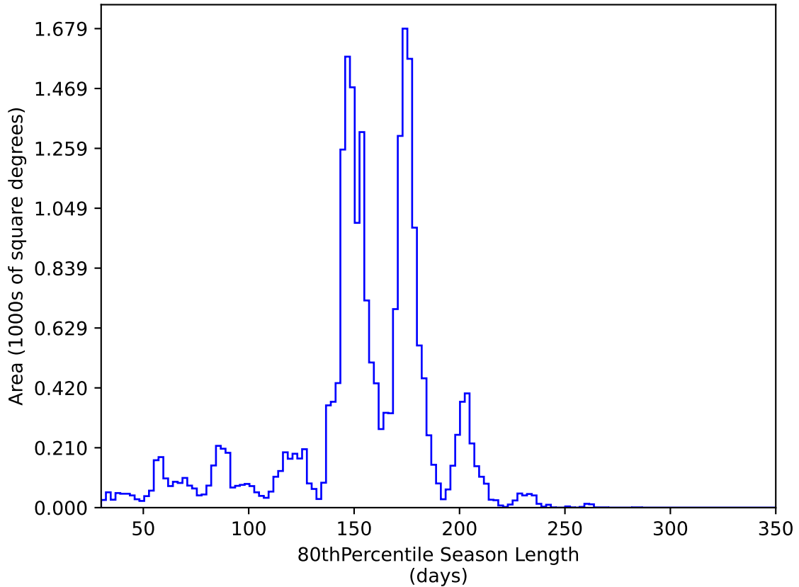
ddf_acor_sf15_lsf20_lsr50_v3.4_10yrs All sky y band: 80thPercentile Season Length
