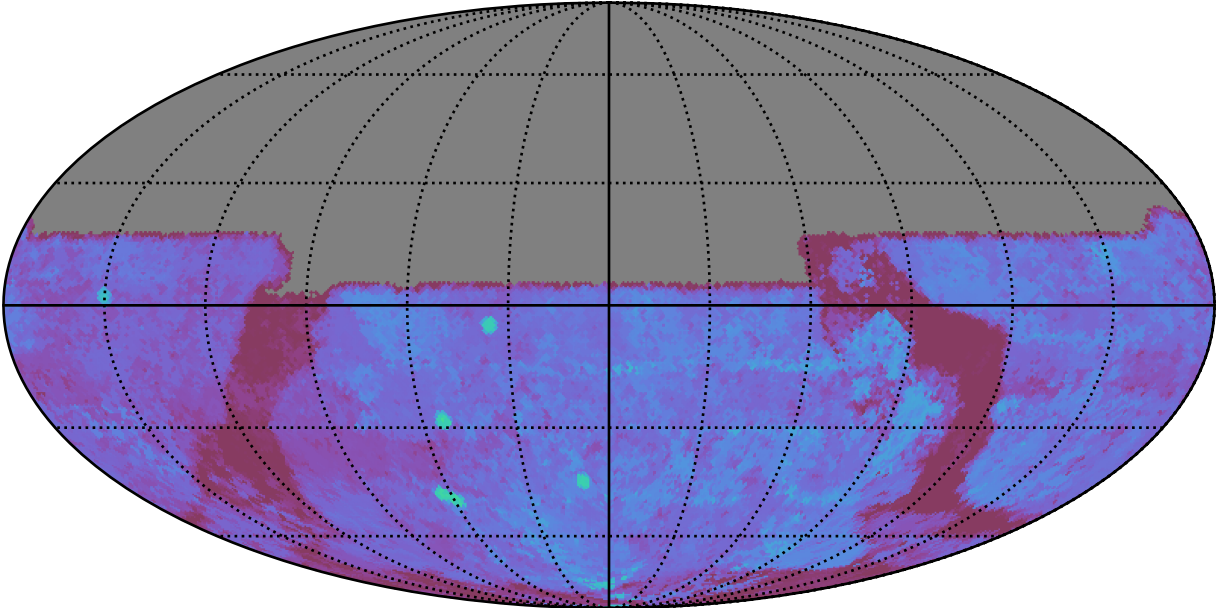
ddf_acor_sf15_lsf20_lsr50_v3.4_10yrs All sky u band: 80thPercentile Season Length
