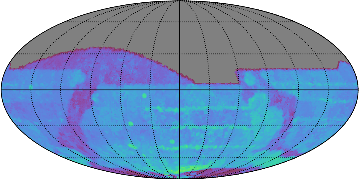
ddf_acor_sf15_lsf20_lsr50_v3.4_10yrs All sky r band: 80thPercentile Season Length
