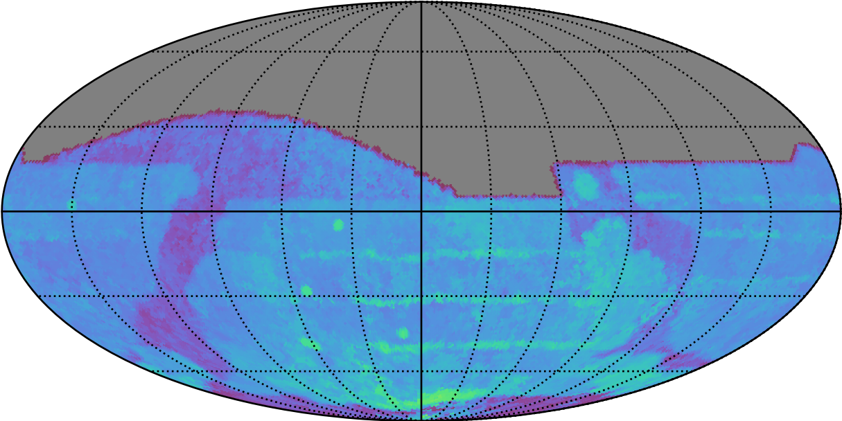
ddf_acor_sf15_lsf20_lsr50_v3.4_10yrs All sky i band: 80thPercentile Season Length
