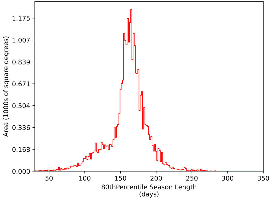
ddf_acor_sf15_lsf20_lsr50_v3.4_10yrs All sky i band: 80thPercentile Season Length
