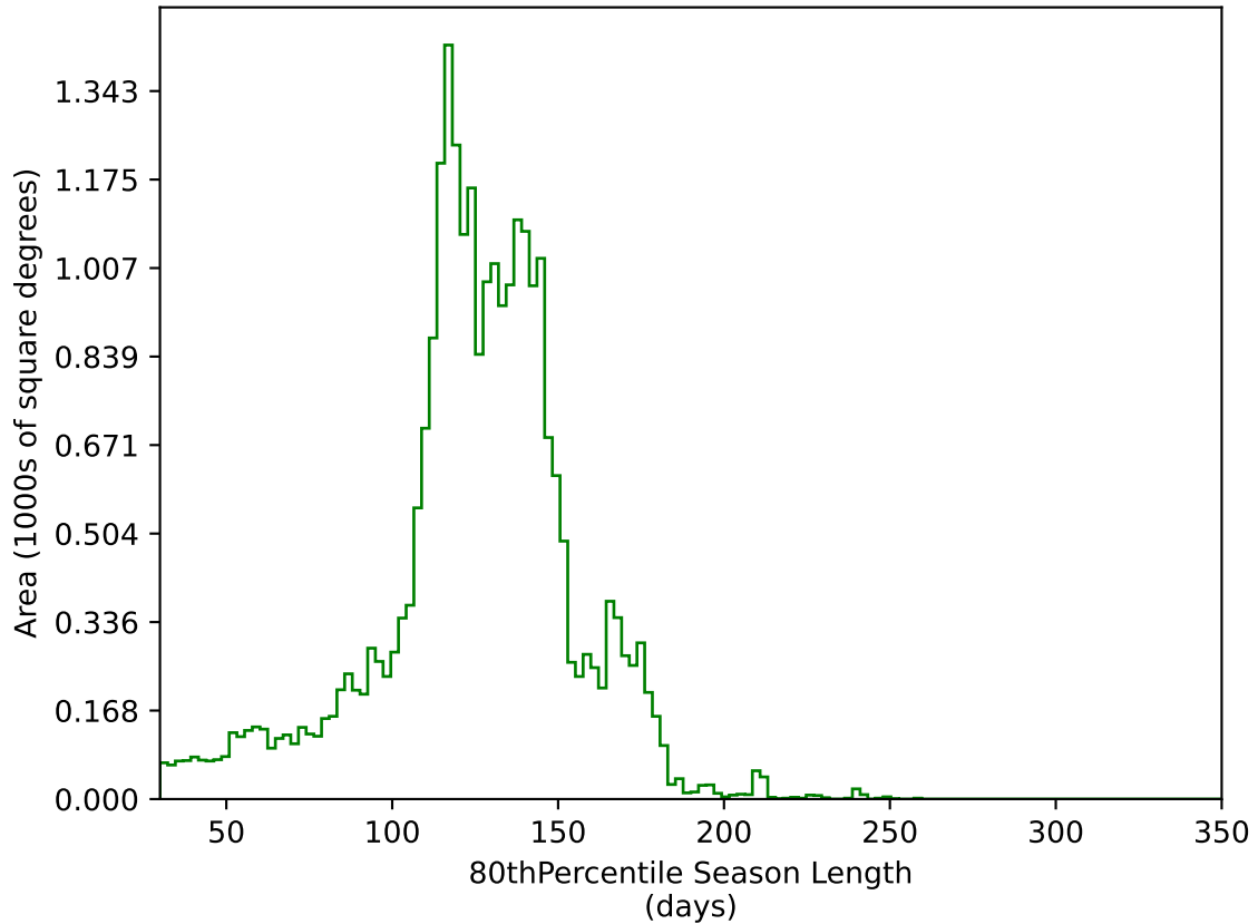
ddf_acor_sf15_lsf20_lsr50_v3.4_10yrs All sky g band: 80thPercentile Season Length
