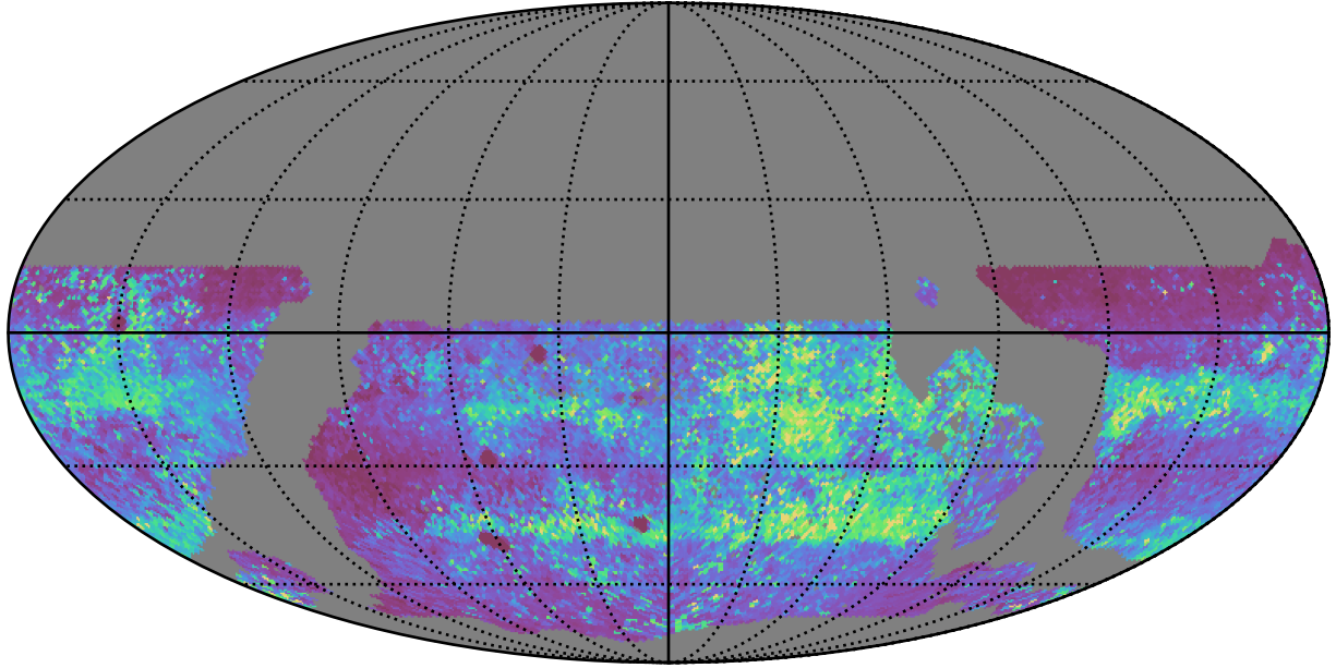
ddf_acor_sf15_lsf20_lsr50_v3.4_10yrs WFD zy bands: 75th Percentile Intranight Timespan
