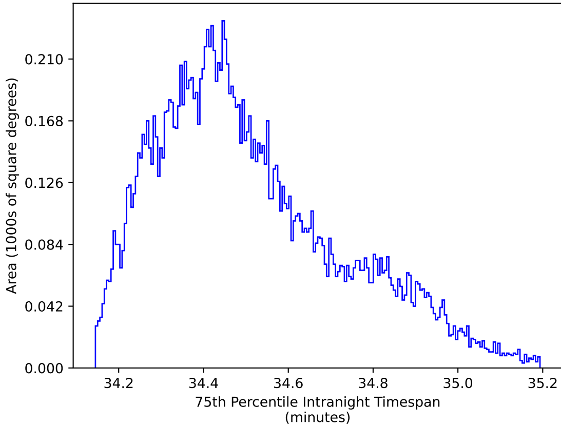
ddf_acor_sf15_lsf20_lsr50_v3.4_10yrs WFD zy bands: 75th Percentile Intranight Timespan
