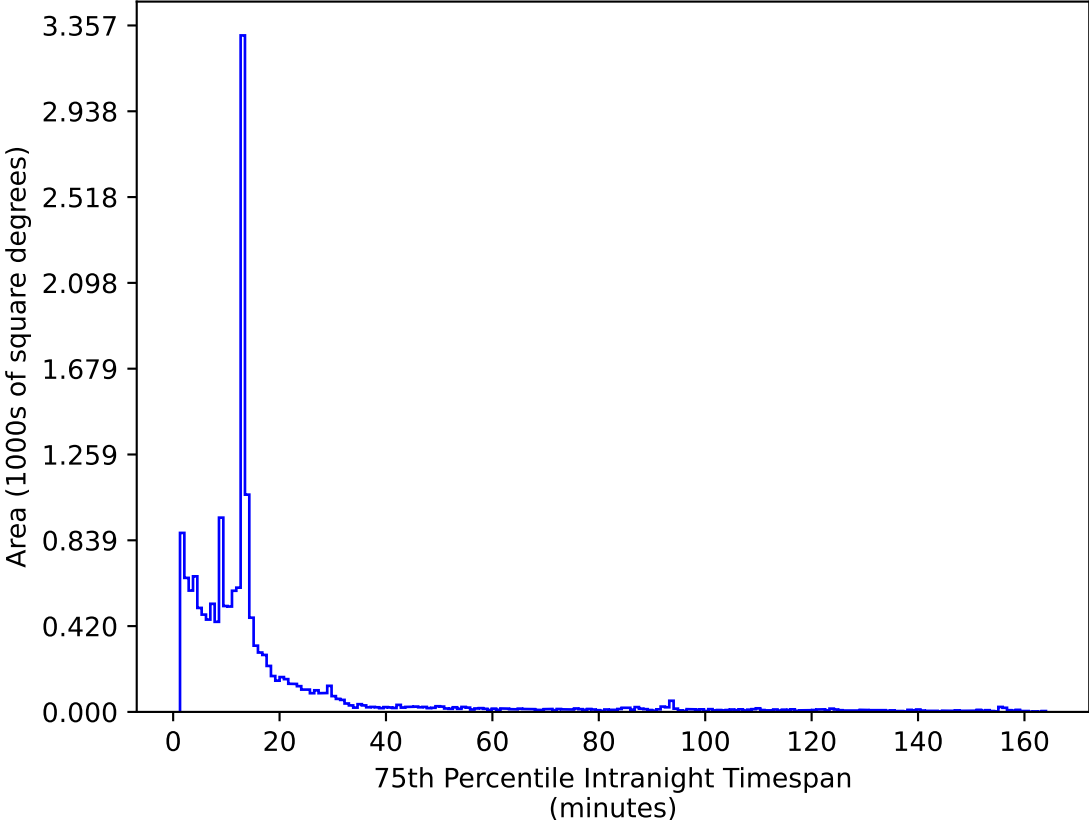
ddf_acor_sf15_lsf20_lsr50_v3.4_10yrs WFD z band: 75th Percentile Intranight Timespan
