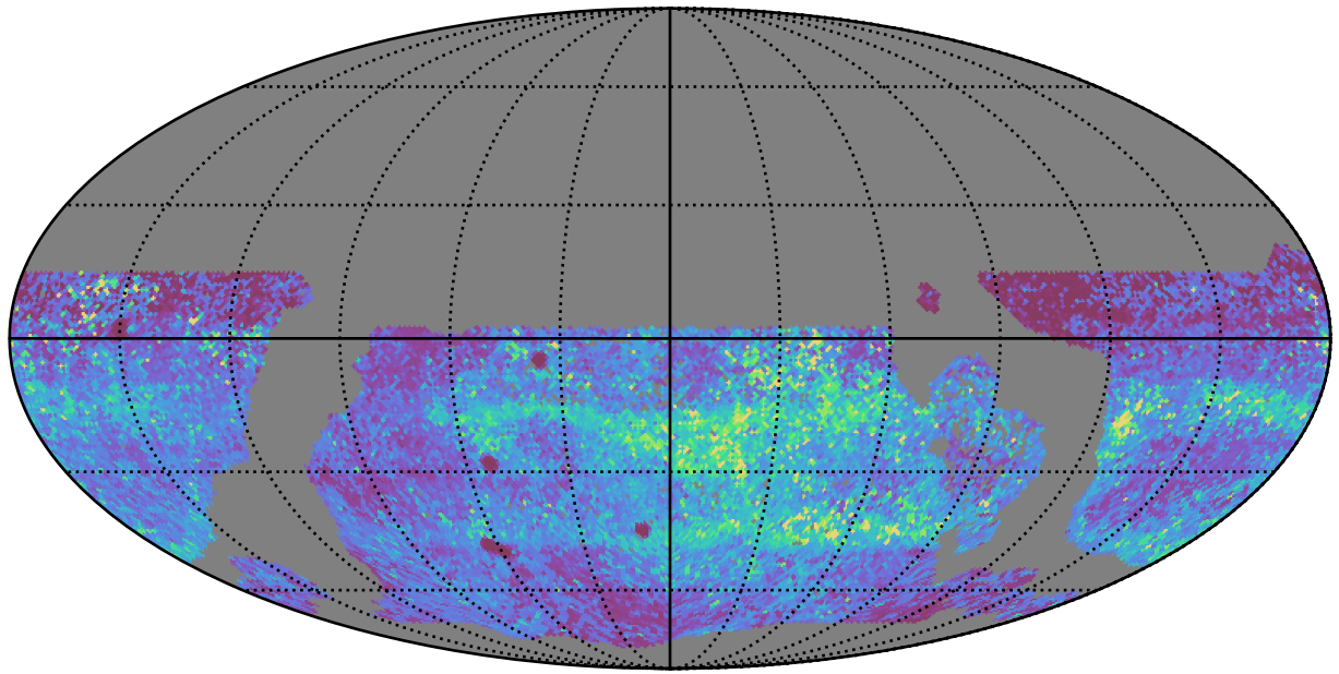
ddf_acor_sf15_lsf20_lsr50_v3.4_10yrs WFD y band: 75th Percentile Intranight Timespan
